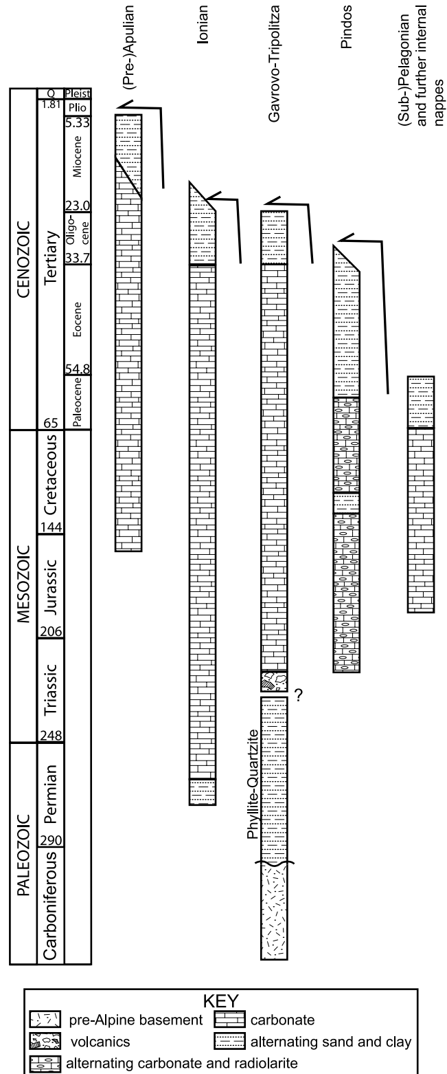
Figure 4. Schematic scheme of the lithostratigraphy of the nappes and timing of nappe emplacement, based on De Mulder [1975], Fleury [1975], IGRS-IFP [1966], Meulenkamp [1982], and Pe-Piper [1982].
