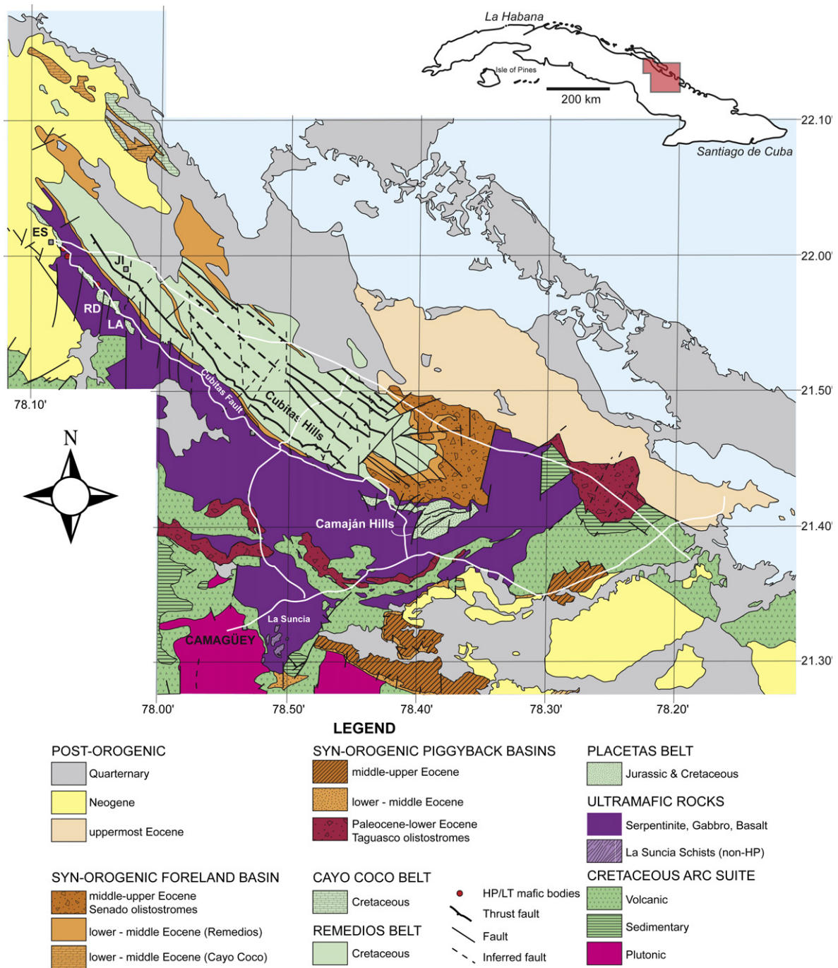
Fig. 2. Geological map of the Camagüey region, central Cuba, compiled from Iturralde-Vinent et al. (1981) and Iturralde-Vinent and Thieke (1986). BA, Banao; ES, Esmeralda, JI, Jiquí, RD, Reforma-Donato block; LA, Las Amarillas block.
