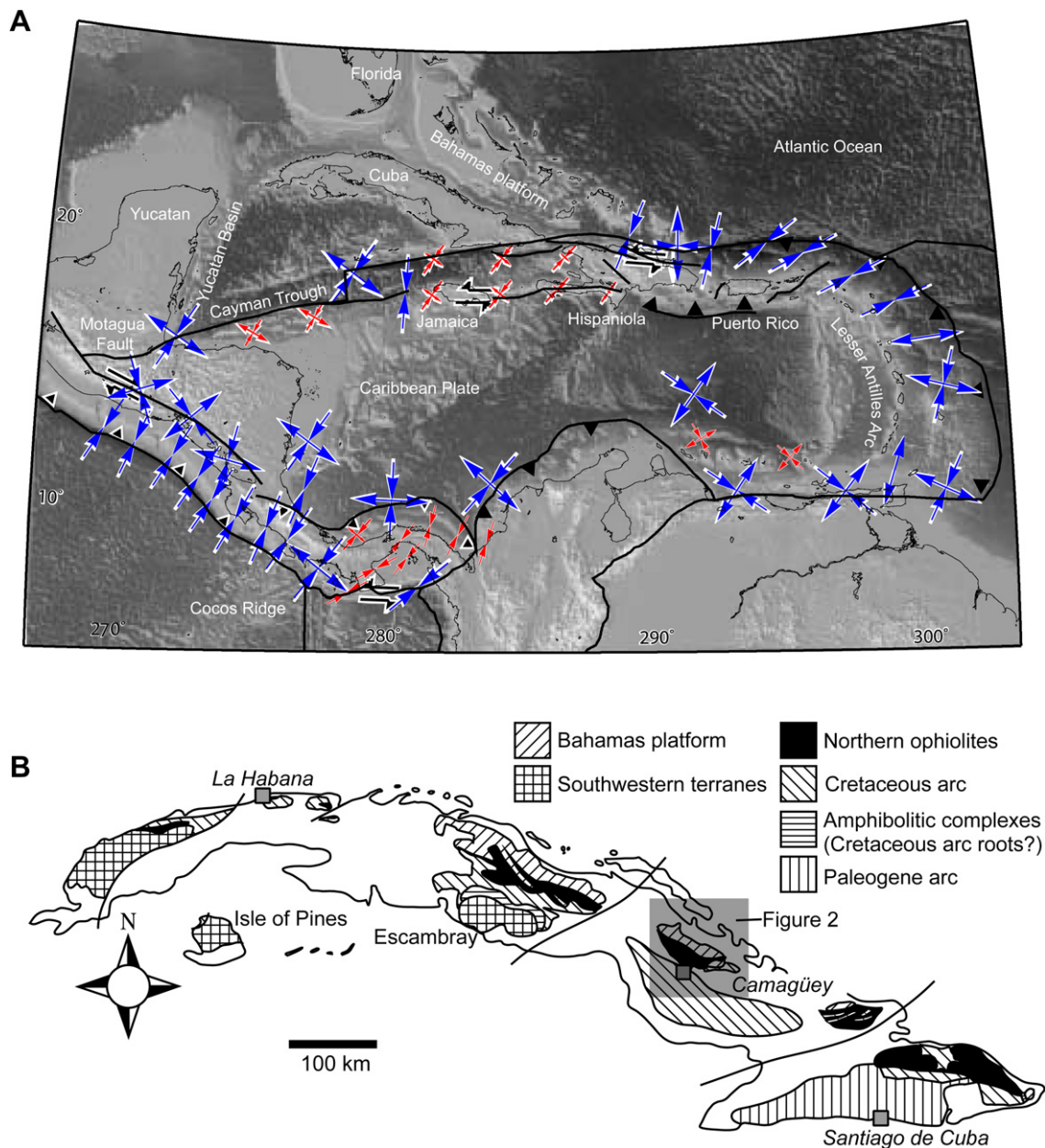
Fig. 1. (a) Tectonic setting of the Caribbean plate. Major tectonic elements and faults: AF, Anegada Fault; AR, Aves Ridge; BP, Bahamas Platform; BR, Barracuda Ridge; CB, Colombia Basin; CR, Cocos Ridge; CT, Cayman Trough; EPGF, Enriquillo Plantain Garden Fault zone; GB, Grenada Basin; HF, Hispaniola Fault zone; MB, Maracaibo Basin; MT, Muertos Trough; MR, Main Ridge; MS, Maracaibo Subduction zone; PTB, Panama Thrust Belt; SSF, San Salvador Fault zone; AF, Anegada Fault; SF, Septentrional Fault zone; HF, Hispaniola Fault zone; PGF, Plantain Garden Fault zone; SF, San Salvador Fault zone; PTB, Panama Thrust Belt; CT, Cayman Trough; GB, Grenada Basin; CR, Cocos Ridge; BR, Barracuda Ridge; MR, Main Ridge; TR, Tiburon Ridge; MB, Maracaibo Basin; MS, Maracaibo Subduction zone; BP, Bahamas Platform; VB, Venezuela Basin; CB, Colombia Basin. Interpreted principal stress directions from the World Stress Map Project (Heidbach et al., 2008) are shown in green/blue. Principal strain rate directions from the Global Strain rate model (Kreemer et al., 2003) are shown in red. The inset panel in the lower right shows vertical axis rotation from Kreemer et al. (2003). (b) Schematic geological map of Cuba, modified after Iturralde-Vinent (1994, 1998b).
