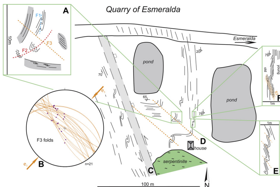
Fig. 8. Form trace map of the Esmeralda block exposed in the quarry west of the village of Esmeralde (Placetas belt; see Fig. 2 for location). Deformation here included at least three phases of folding, illustrated by the outcrop in (A). The structure of the western and eastern side of the quarry cannot be straightforwardly linked, and we infer a fault separating these domains, supported by the jump in the edge of the block in the south, where it is juxtaposed against serpentinite.
