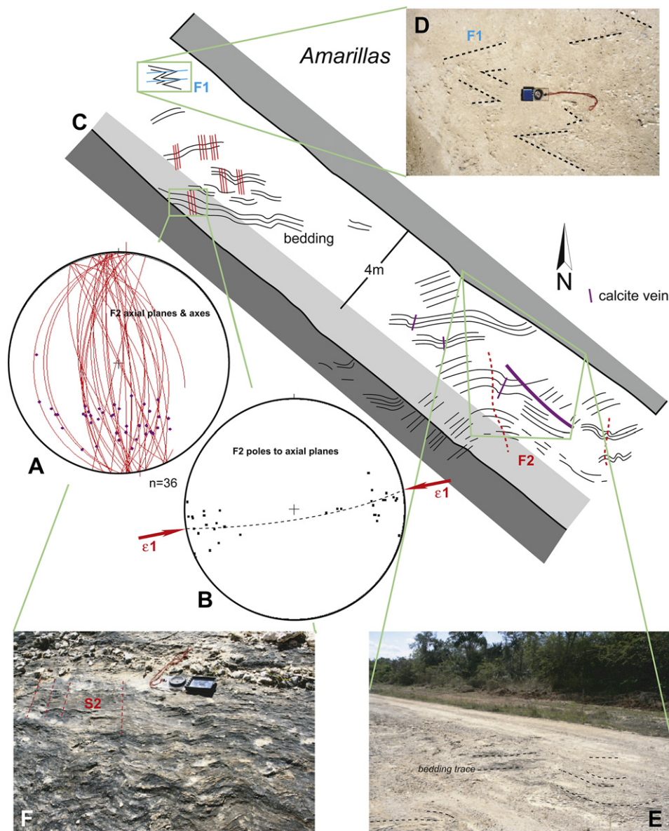
Fig. 6. Form trace map of the small road floor exposure of the Las Amarillas block (Placetás belt; see Fig. 2 for location). The deformation of the Las Amarillas block is characterized by a second phase of open folding and locally associated axial plane cleavage, which overprints a first phase of isoclinal folding. The spread in poles to F2 axial planes and F2 fold axes may indicate a third, weaker phase of folding, the shape of which cannot be constrained in this outcrop. (E) The typical outcrop used for study of the structure.
