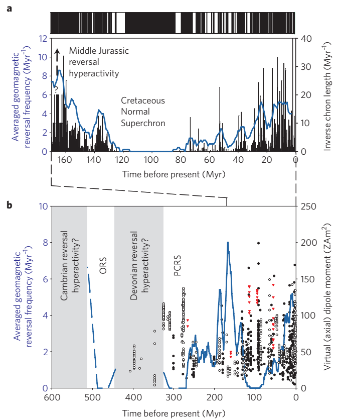
Figure 1 | Records of geomagnetic polarity reversal frequency and dipole moment since the Cambrian period.
