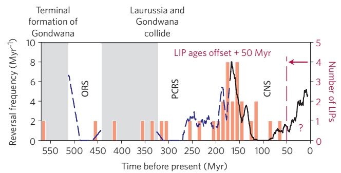
Figure 3 | Average reversal frequency and eruption ages 20 of large igneous provinces (LIPs; offset by +50 Myr) that have not yet been subducted.
