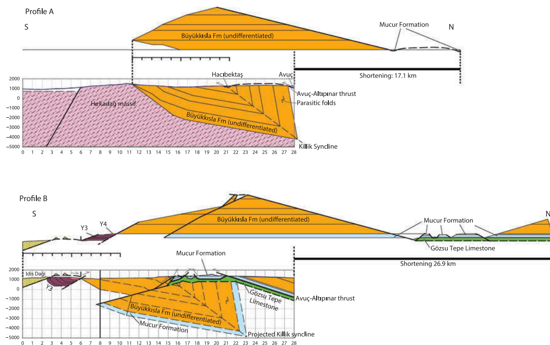
Figure 9. Structural profiles A and B and their restorations. See Figure 4 for locations of the profiles. Büyükkışla Formation and Muçur Formation are not further subdivided into members.
