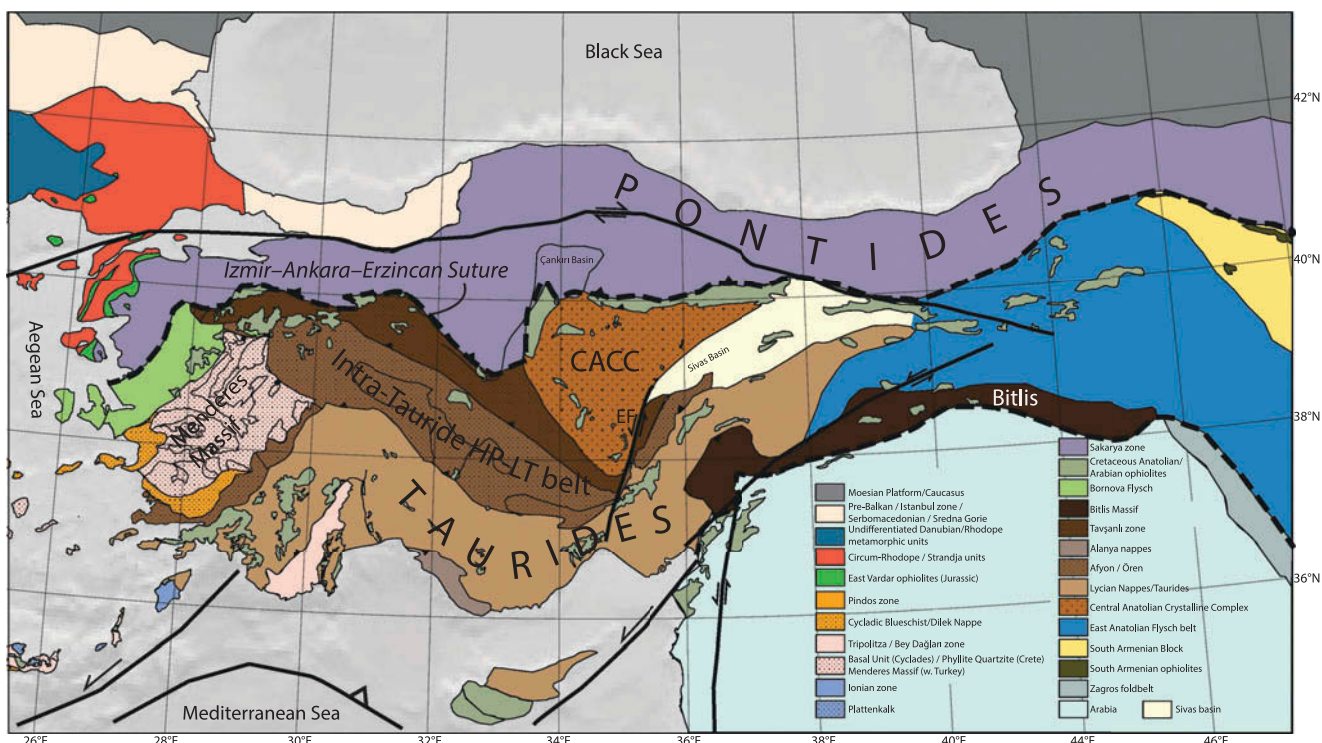
Figure 1. Tectonic map of the eastern Mediterranean region, modified after Okay et al. (1996), Şengör et al. (2008), Pourteau et al. (2010), and van Hinsbergen and Schmid (2012). EF = Eciş Fault.
