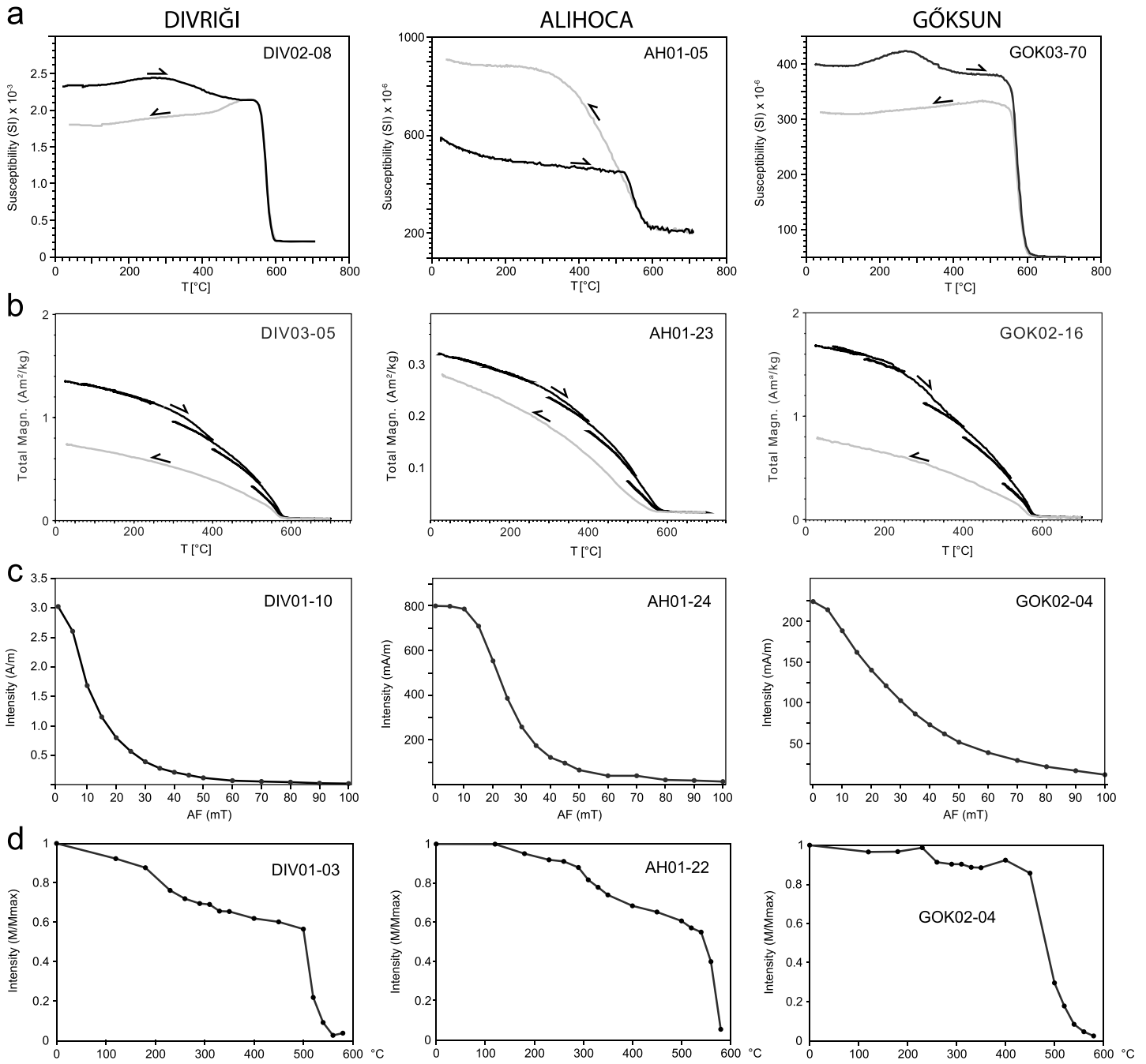
Figure 4. Results from rock magnetic experiments for representative samples from the Divriği, Göksun, and Alihoça ophiolite. (a) Thermal variation of low-field magnetic susceptibility; the black (gray) lines are the heating (cooling) paths. (b) Thermal variation of magnetic remanence during Curie balance experiments; the black (gray) lines are the heating (cooling) paths. (c) Magnetization decay paths during alternating field (AF) demagnetization. (d) Magnetization decay paths (normalized values) during thermal demagnetization.
