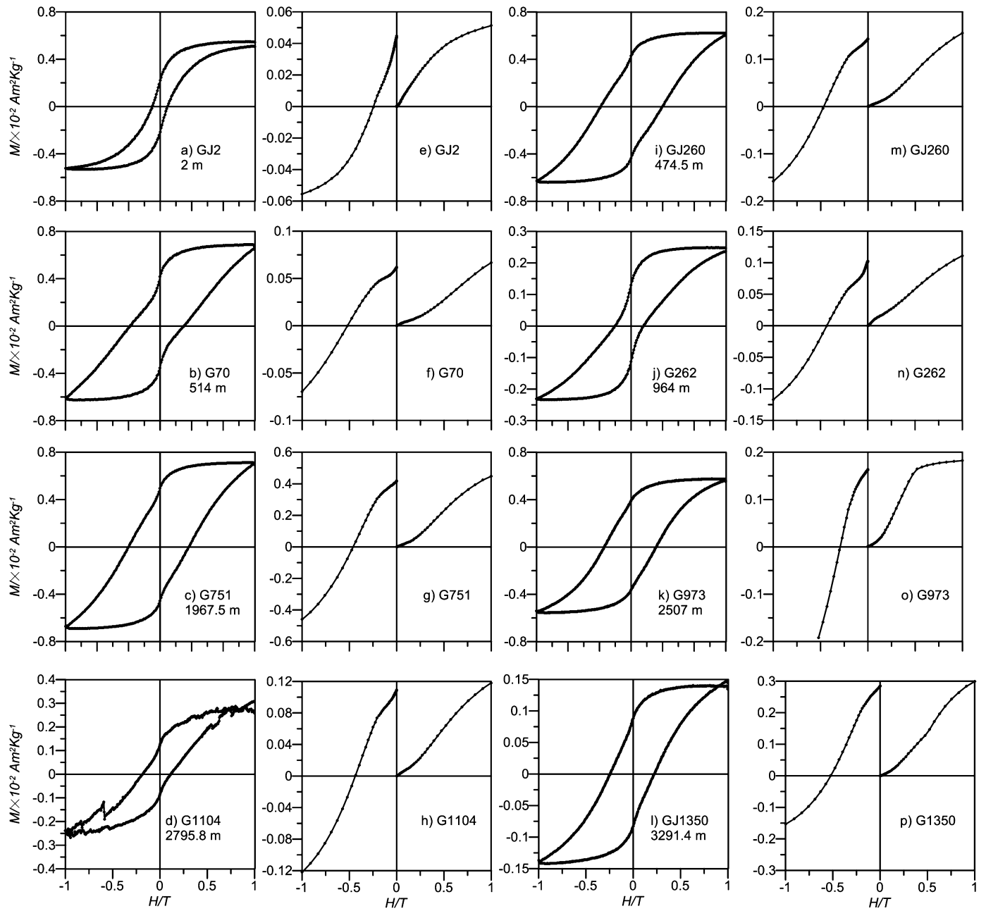
Fig. 3. (a–d, i–l) Hysteresis loops, and (e–h, m–p) IRM acquisition curves and direct current field demagnetization of the saturation IRM from representative sample of the Gonjo Basin.
